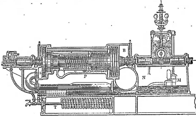
Sectional View of 400 K. W. Westinghouse Turbine
